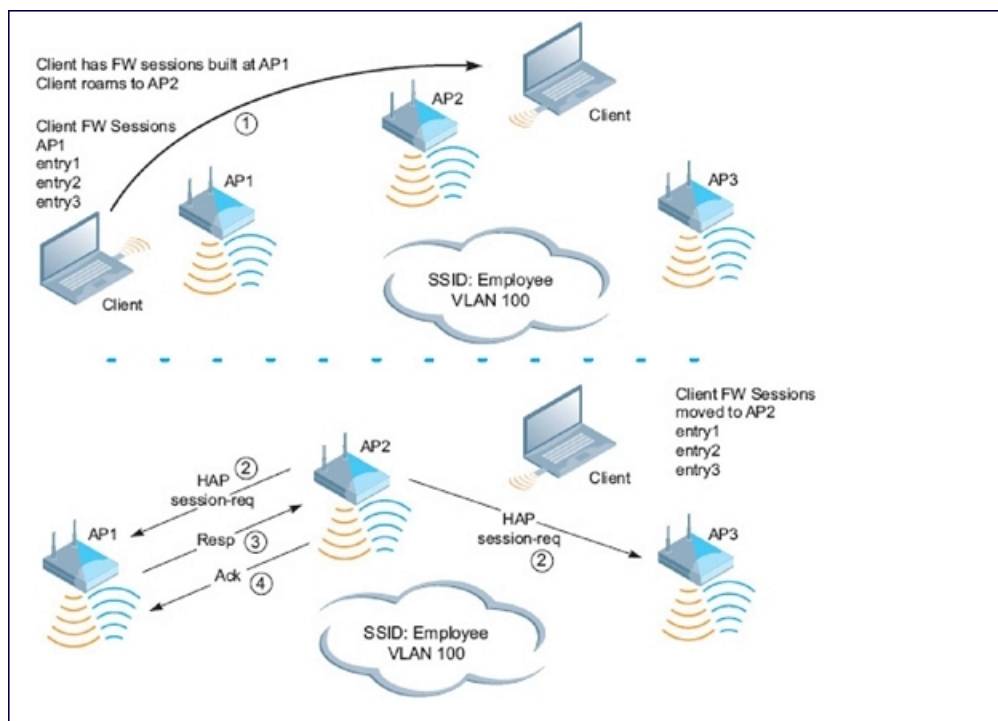
Figure 70 Bridge Mode Mobility
