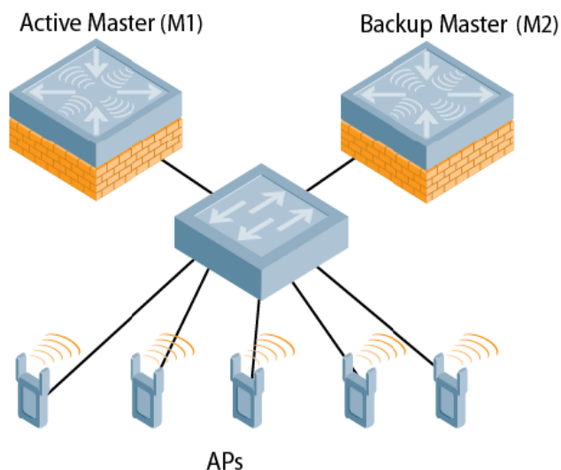
Figure 63 Redundancy with a Active-Backup Master Switch Pair
