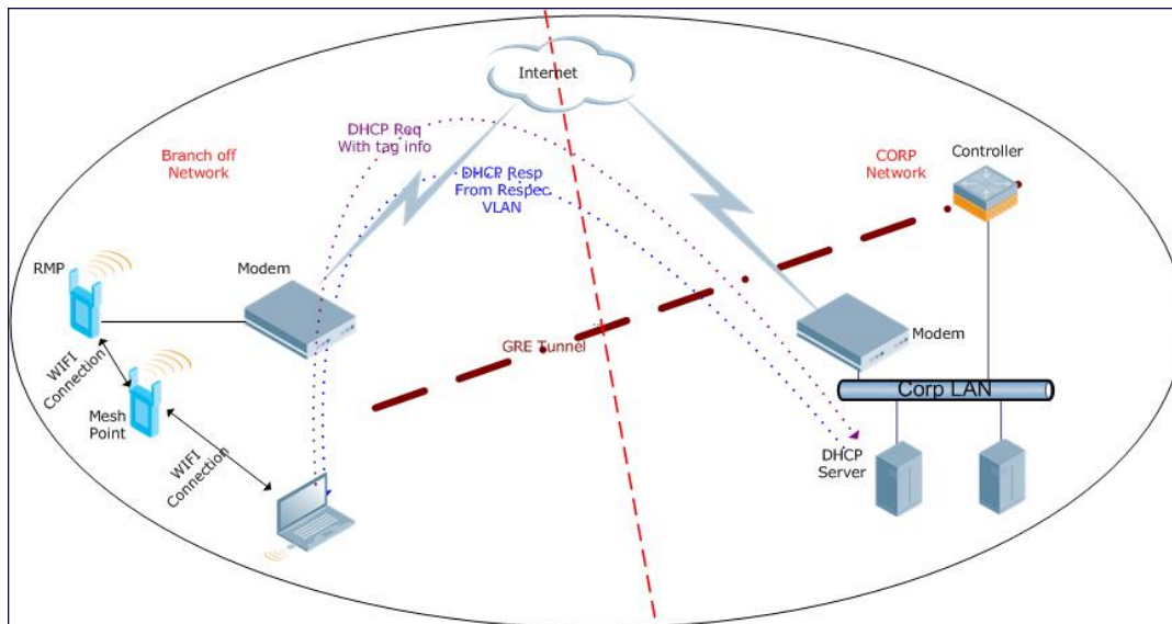
Figure 55 Working of RMP
