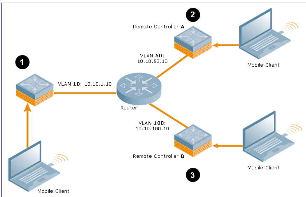
Figure 71 Inter-Switch Mobility
