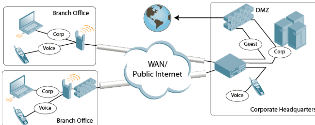
Figure 79 Remote AP with Single Switch
