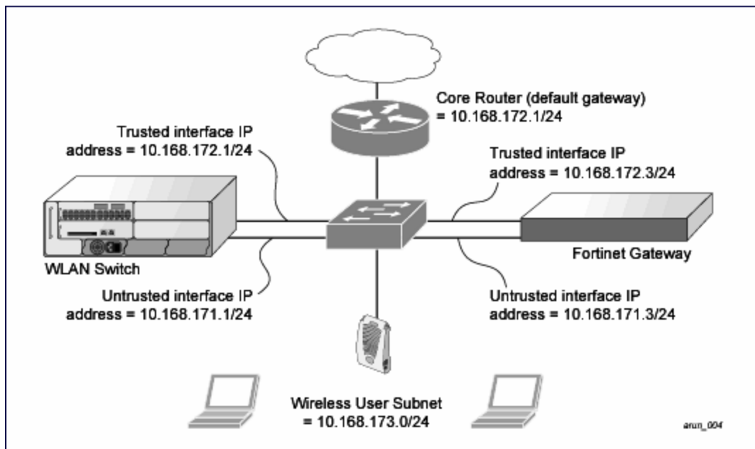
Figure 242 Example Route-Mode Topology
