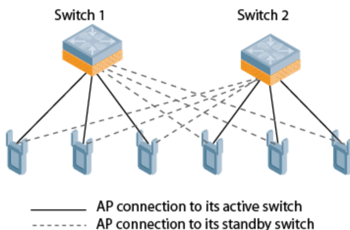
Figure 60 Active-Active HA Deployment
