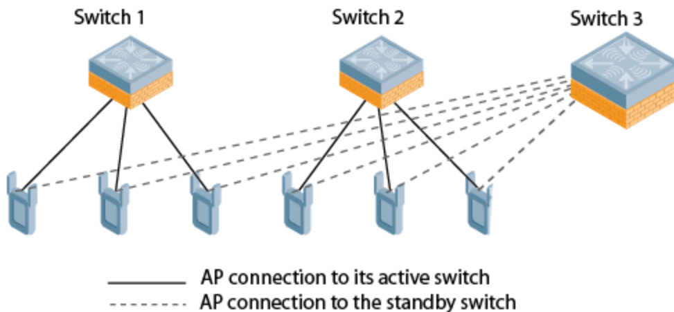
Figure 62 1:1 Active/Standby Deployment
