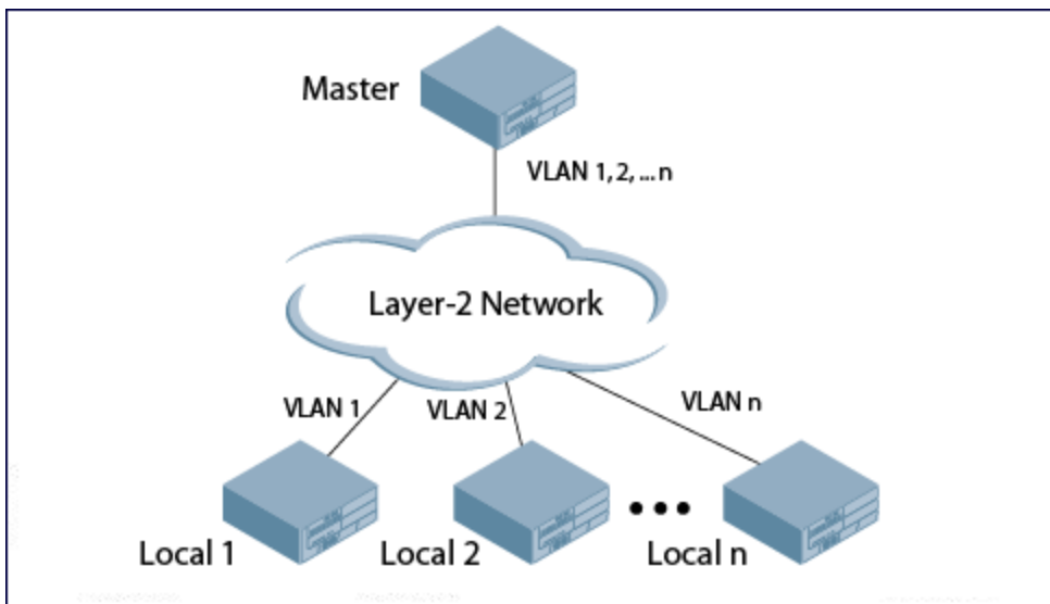
Figure 64 Redundant Topology: Master-Local Redundancy
