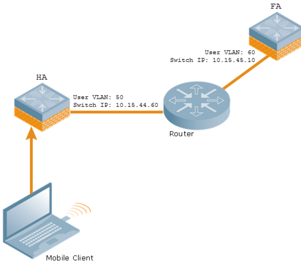
Figure 69 Sample IPv6 L3 Mobility Configuration
