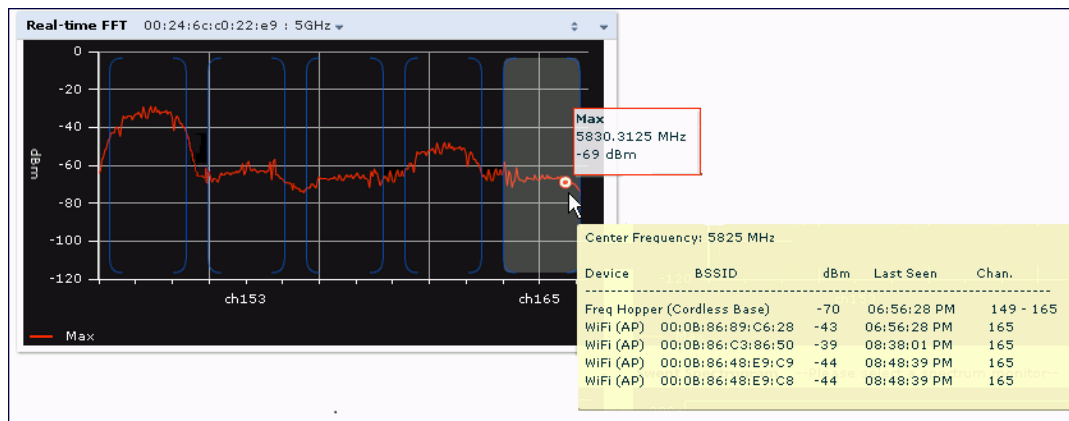
Figure 122 Real-Time FFT
