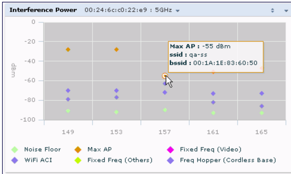
Figure 120 Interference Power
