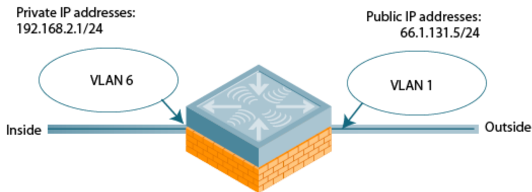
Figure 19 Example: Source NAT using Switch IP Address
