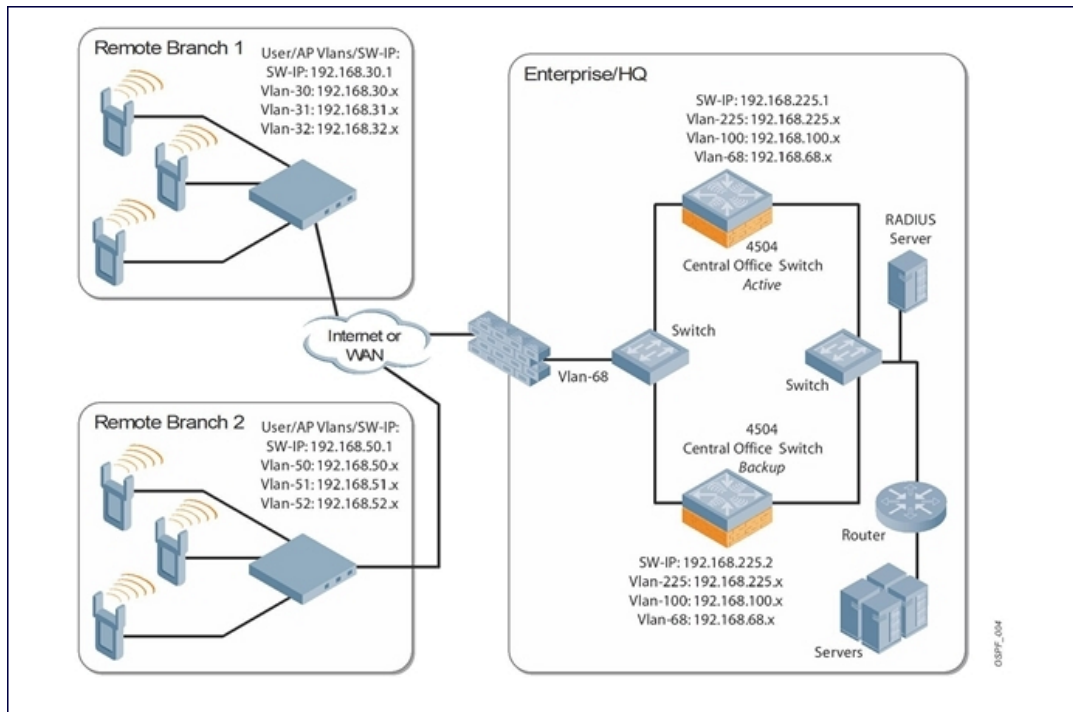
Figure 28 Sample OSPF Topology
